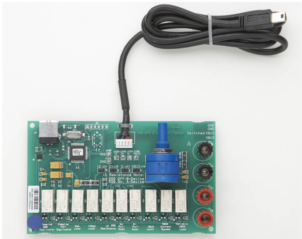
Figure 6 Keysight N5417A USB OTG Test Fixture
