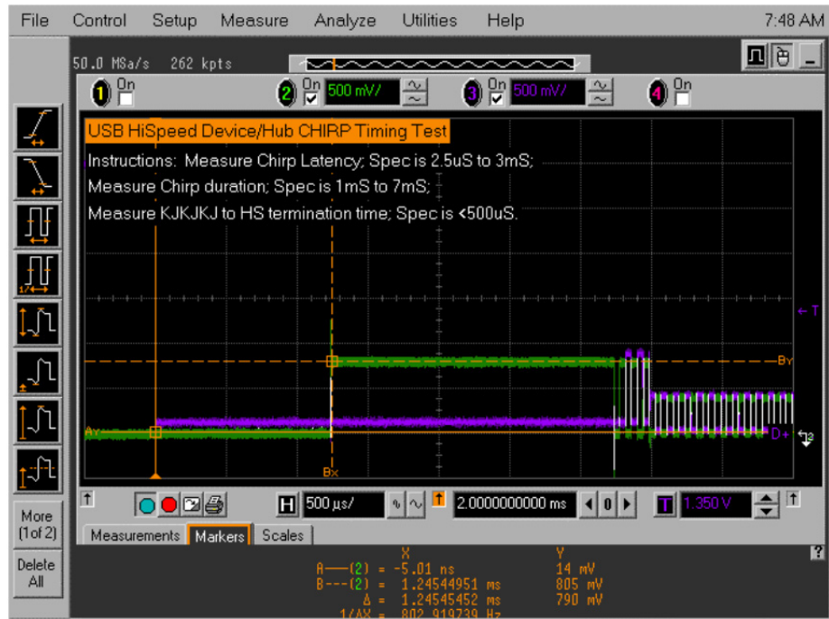
Using the automatic measurement shown in Figure 7, measure the device's CHIRP-K duration.
